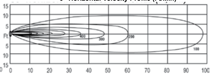
30" Horizontal Velocity Profile (Ft/Min)
